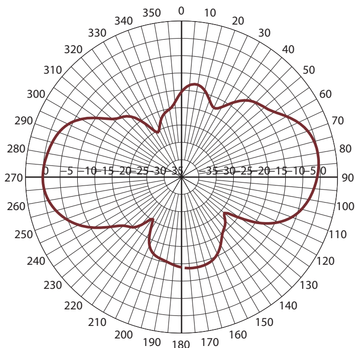
Elevation Pattern @ 5 GHz
