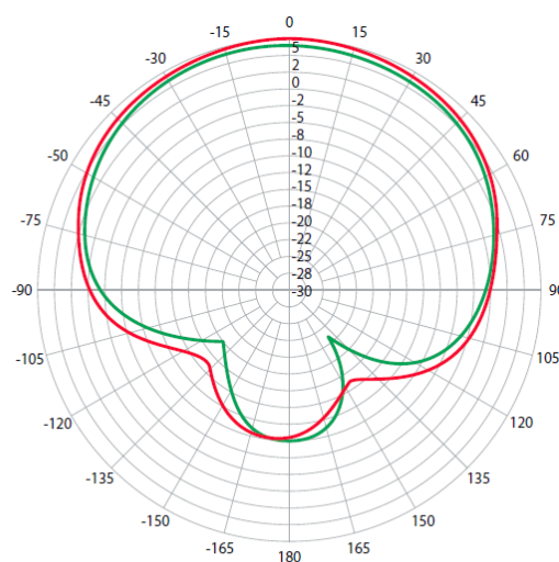
1800 MHz – Azimuth (deg) – Amplitude (dB)
