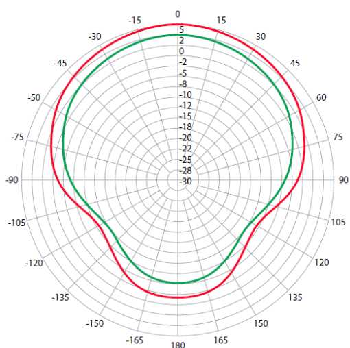
900 MHz – Azimuth (deg) – Amplitude (dB)
