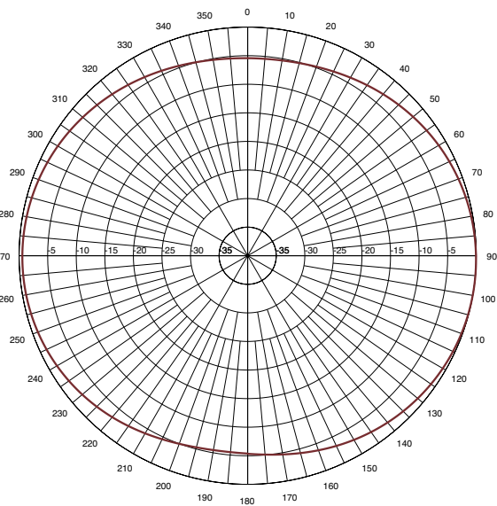
Azimuth Pattern
