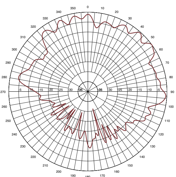
Elevation Pattern
