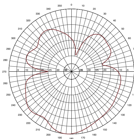
Azimuth Pattern
