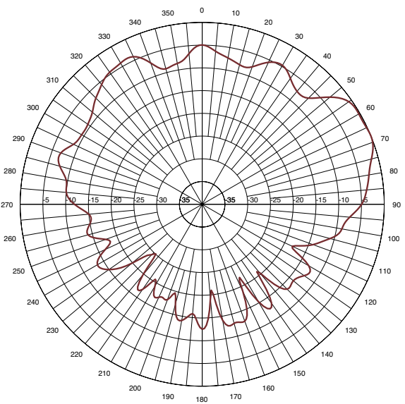
Elevation Pattern
