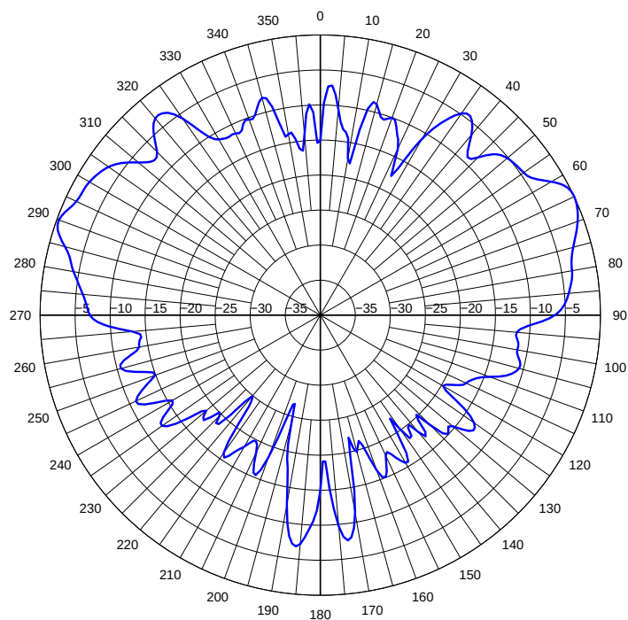
2 GHz Elevation Pattern
