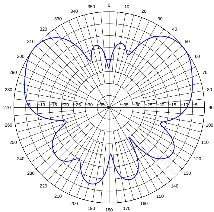
750 MHz Elevation Pattern
